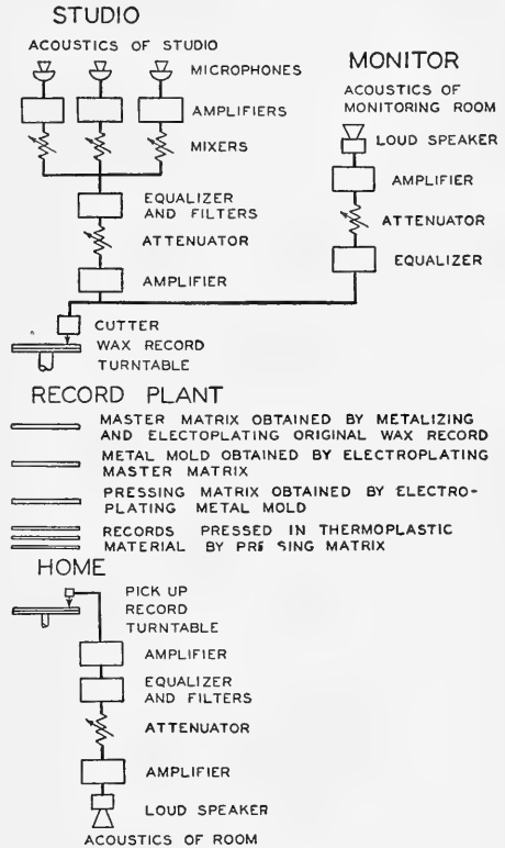
FIG. 12.22. Complete phonograph recording, record pressing and reproducing system.
